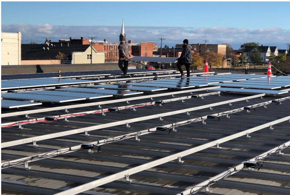
Jolma Electric employees installing solar panels
